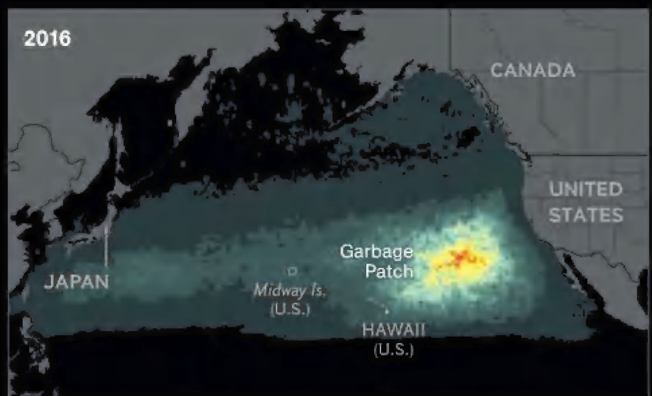
This five-year projection shows how debris from Japan’s 2011 earthquake and tsunami disaster is likely to spread via the North Pacific Subtropical Gyre, a clockwise spiral of currents.
